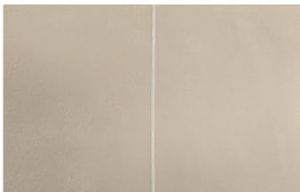
Limestone
