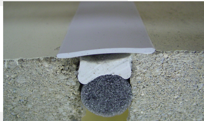
Cross section of sealant joint repaired with Simple Seal
