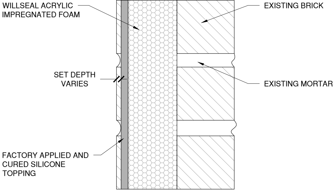
1 SECTION VIEW
