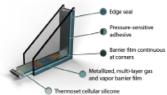
Typical glazed application of spacer
