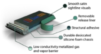
EnerEDGE warm-edge spacer
