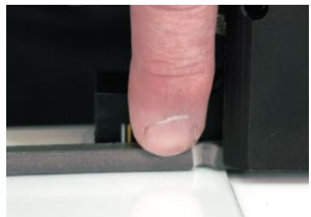
Tacking behind corner notch
